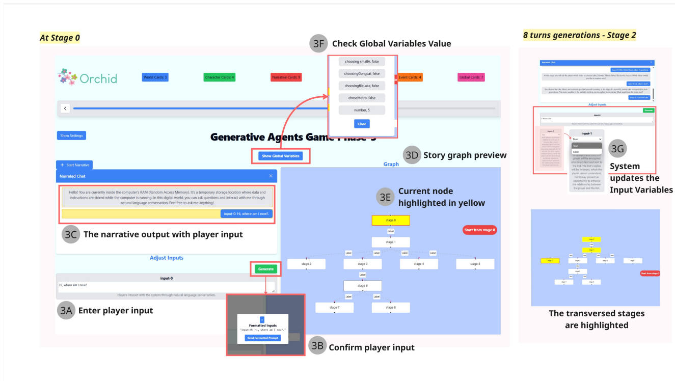
Figure 5: Interactive process of phase 3. The author can simulate user input (3A) and generate the corresponding narrative (3B, 3C). The story graph (3D) shows the current narrative node (3E). The author can check whether the Global Variables are updated appropriately (3F). Upon triggering the transition through player inputs, the story graph and player input are updated (3G).
