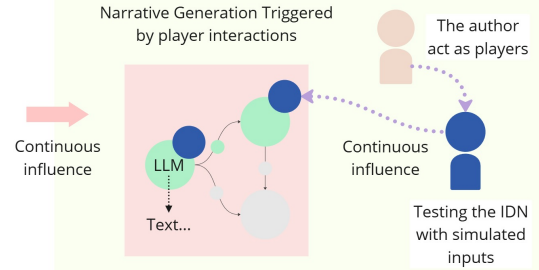
Figure 1: Overview of Orchid-Creator . Authors construct LLM-driven IDNs through two phases. In phase (A), they design the story graph, including in-node interactions and transitions, resulting in a static LLM-driven IDN framework. In phase (B), authors simulate player input to test the IDN created in Orchid-Creator .
